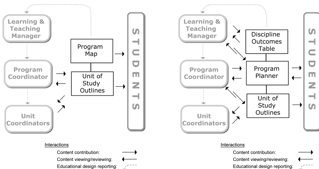
Figure 2: Information flow in Version 1 Database
